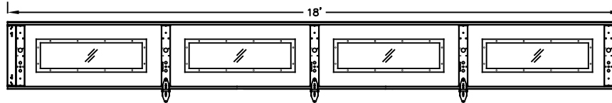
LONG LITE GLAZING LAYOUT
