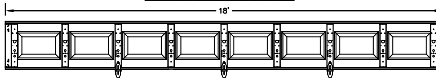
CENTER STILE & INTERMEDIATE HINGE LOCATIONS
